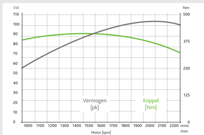
↑ vermogenscurve 4100E.
