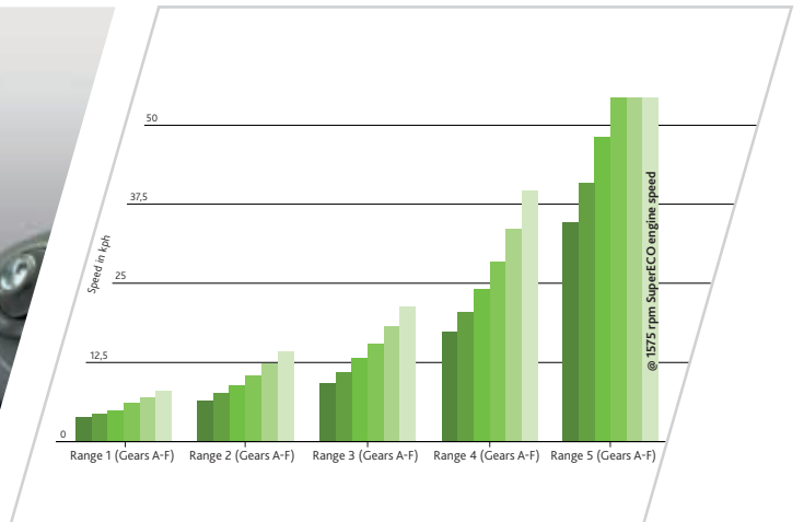
> RCshift speeds: exceptional overlap of the different ranges and 50 kph superECO for maximum fuel efficiency (engine rpm with maximum tire size).
