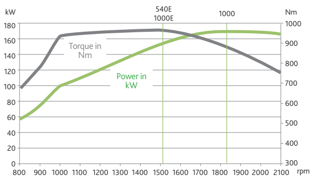
> Low engine speed concept with optimised power and torque curves (6230 TTV - 6230 TTV HD curve shown in graph).
