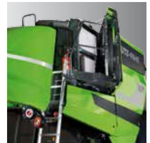
All radiators can be opened like a book and immediately accessed for periodic cleaning.
